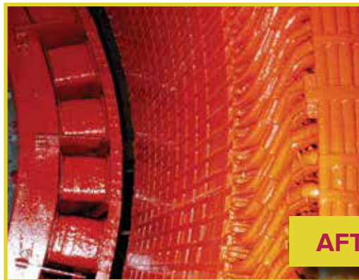
On-Site Recondition of (6) 3,000 HP 4 kV Ball Mill Motors with Before and After Dry Ice Cleaning Results
